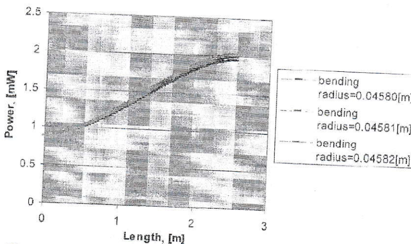
Fig. 2 – EDFA bending effect simulation, for a doped fiber, single step, with radius=1.7 \mu m and doping density=1.22 \times 10^{25} /m ^3 .
