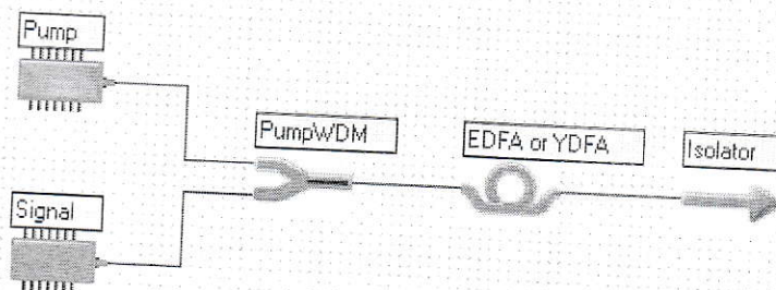
Fig. 1 – Standard Fiber Amplifier Setup for Bending Measurement (LAD 4.0 license).
